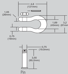
Standard Shackle
