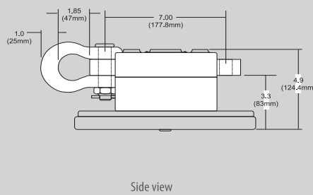
Standard Shackle
